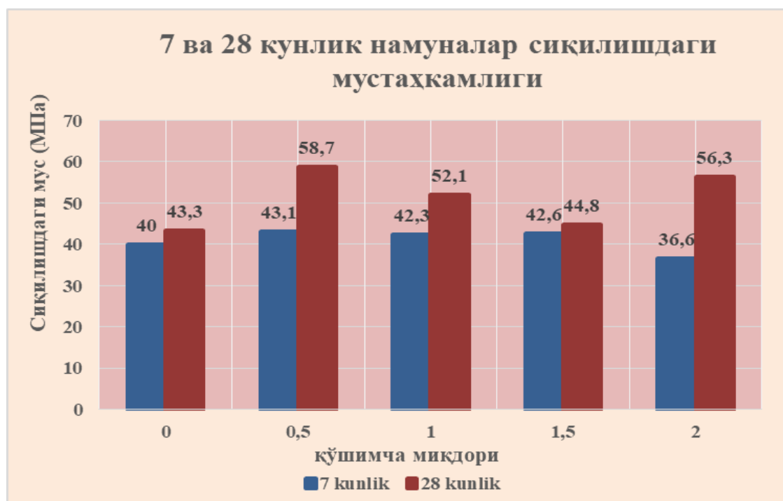
Figure-1. “Betong strong-17” the effect of the additive on the compressive strength of concrete.
